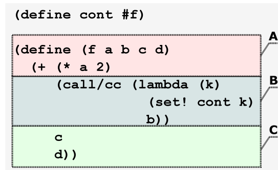
Рис. 6.2. call-with-current-continuation
